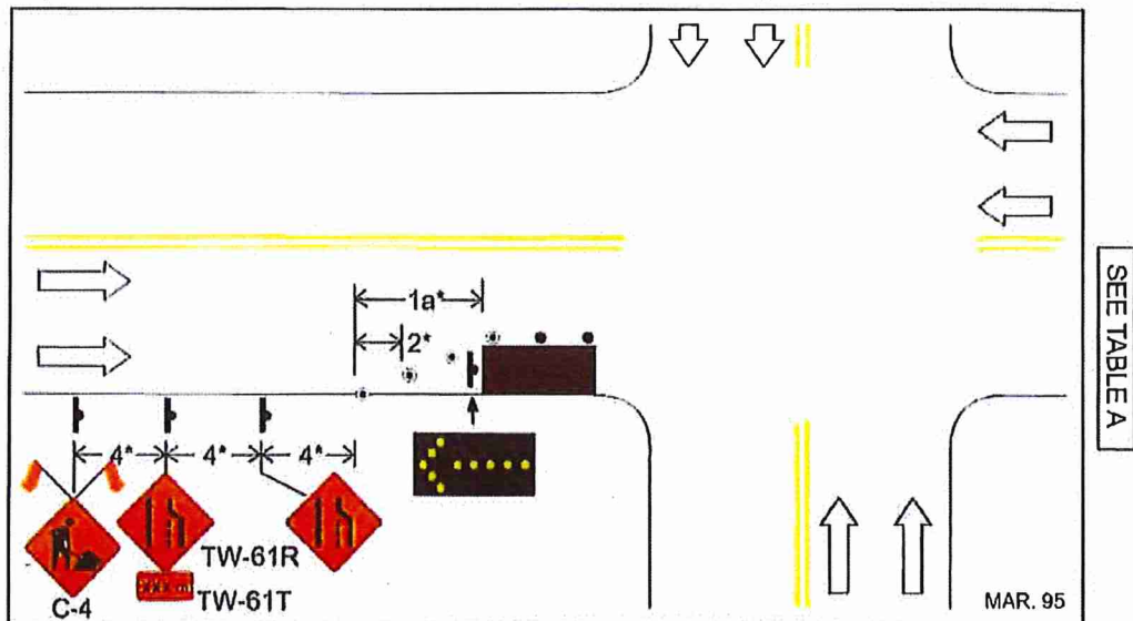
Figure 3.4.3 Right Lane Closed – Multilane Roadway
